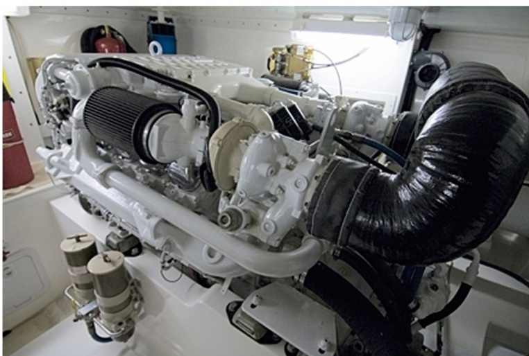
engineroom2_starboard_engine.jpg
