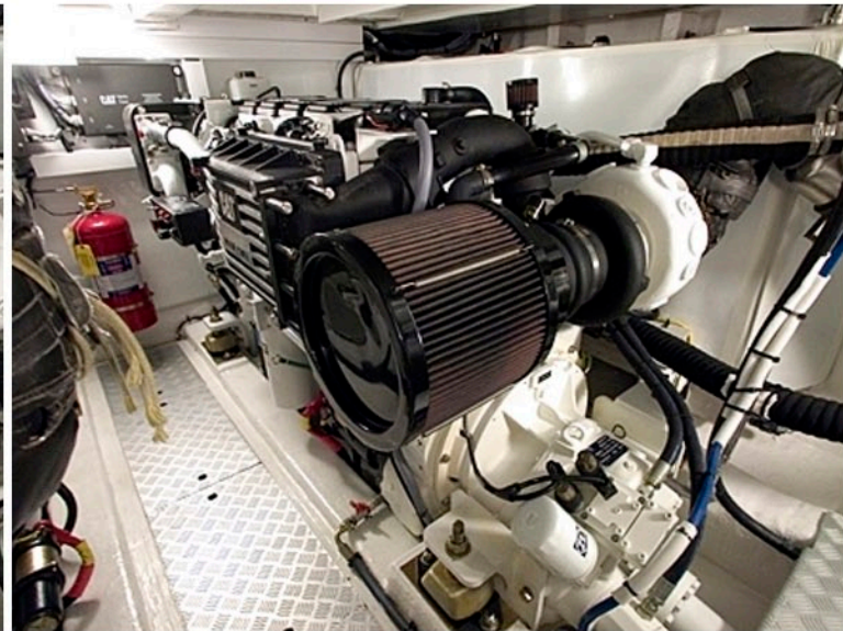
engineroom2_starboard_engine.jpg
