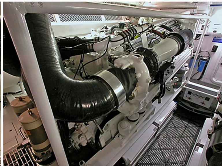
engineroom3_port_engine.jpg
