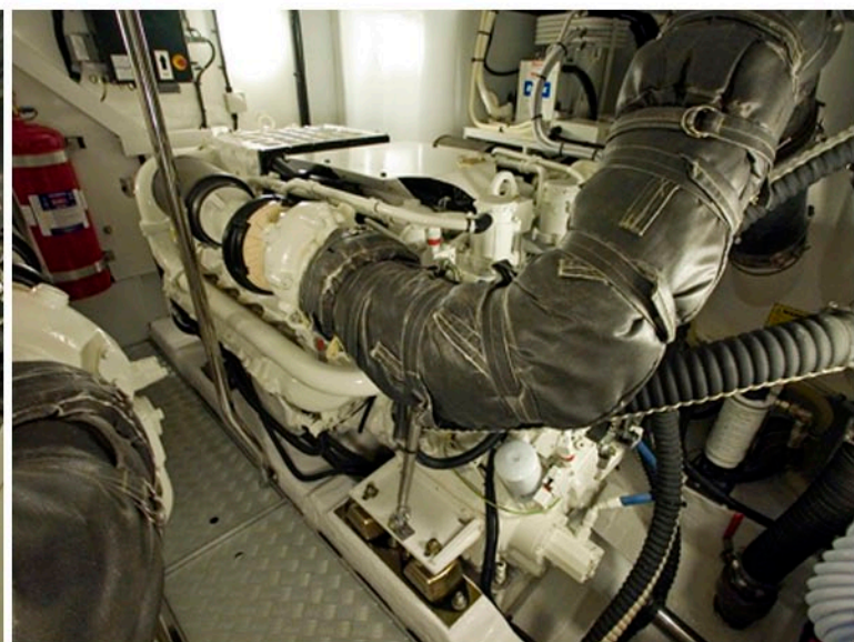
engineroom2_starboard_engine.jpg
